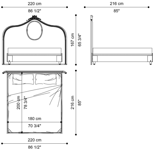
BED J.GLR-02
