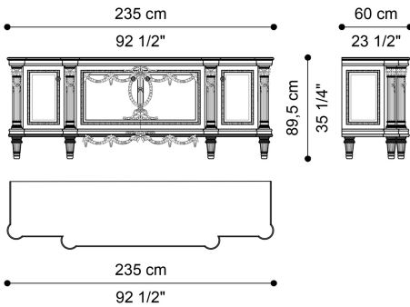
SIDEBOARD J.GLR-11B
