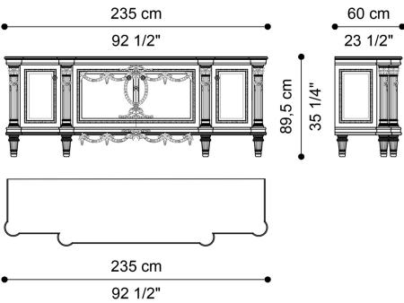
SIDEBOARD J.GLR-11
