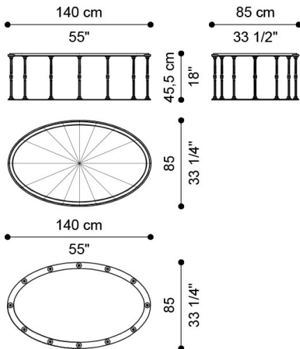
LOW TABLE J.LUM-176
